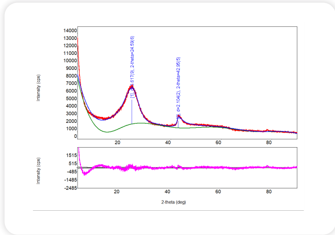
AEROFEN Reduced Graphene Oxide XRD Results
