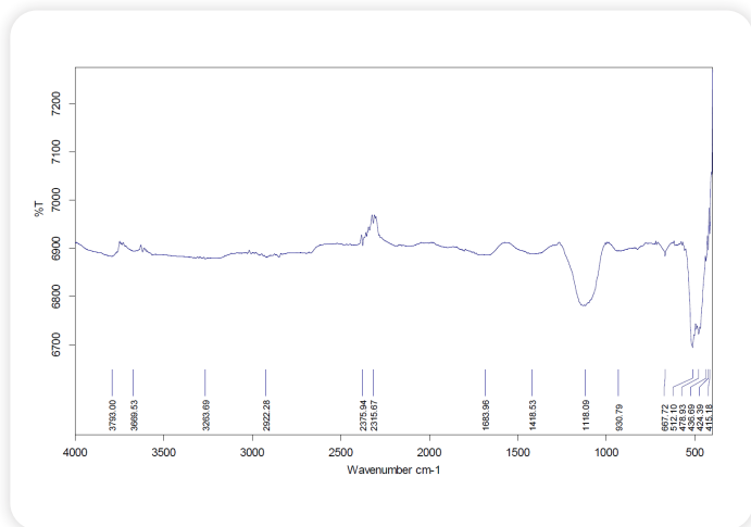
AEROFEN Reduced Graphene Oxide FTIR Results
