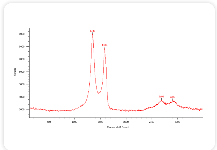
AEROFEN Reduced Graphene Oxide RAMAN Results
